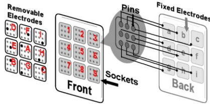
Fig 4. Design of a reconfigurable CipherCard.
