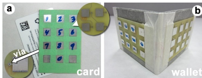
Fig. 2. Left: Card-shaped CipherCard with a 3 \times 4 electrode grid. Top callout shows the internal wiring and bottom callout shows the via and electrodes on the back. Right: Wallet-based CipherCard.
