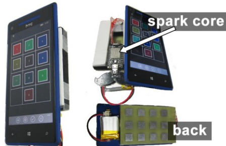
Fig 3. Phone-based CipherCard.
